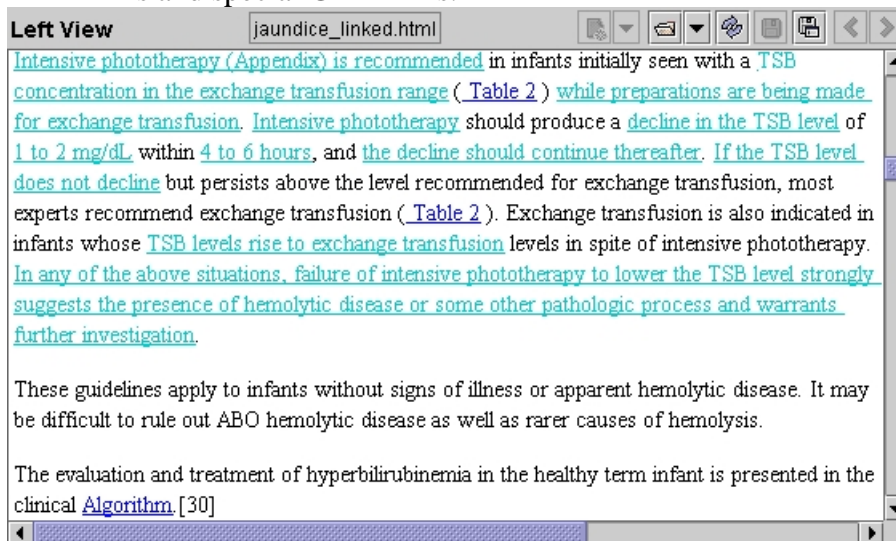
Fig. 14: HTML View
