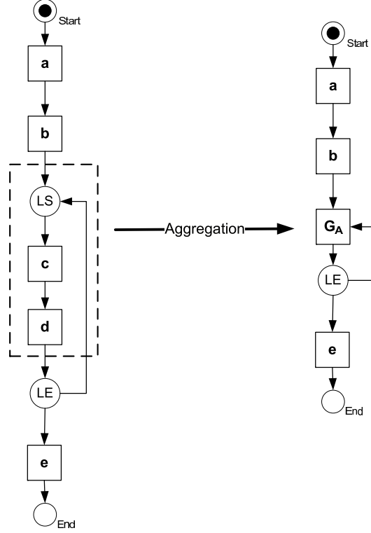
Fig. 5. The counterpart of control nodes must be included in aggregation
