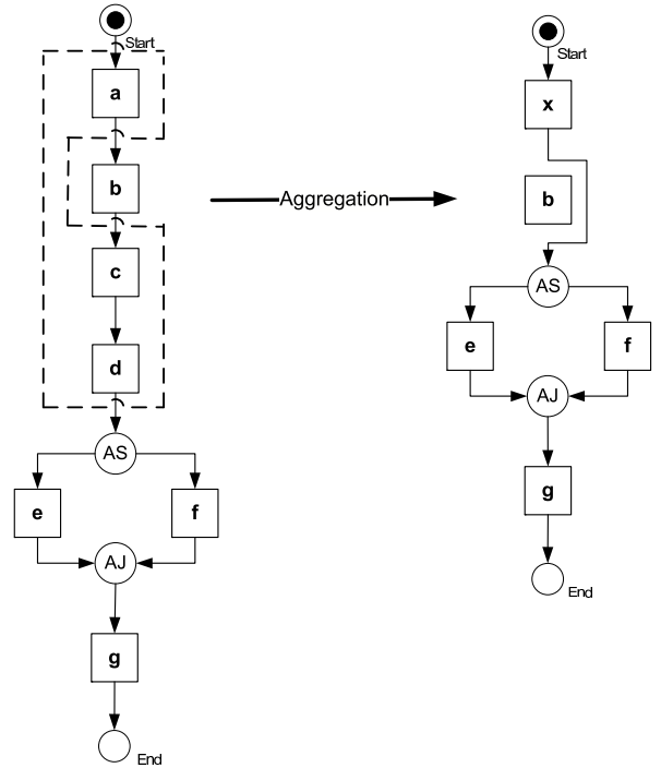
Fig. 3. Aggregated activity is not a connected subgraph
