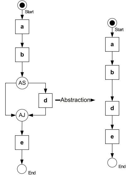
Fig. 2. Application on control nodes
