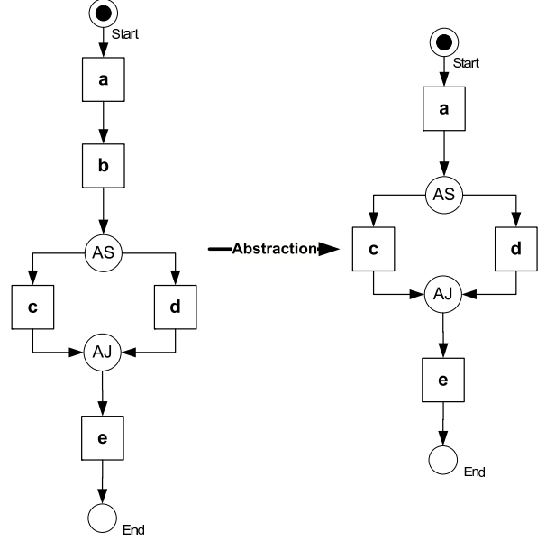
Fig. 1. Application of abstraction on the activity b
