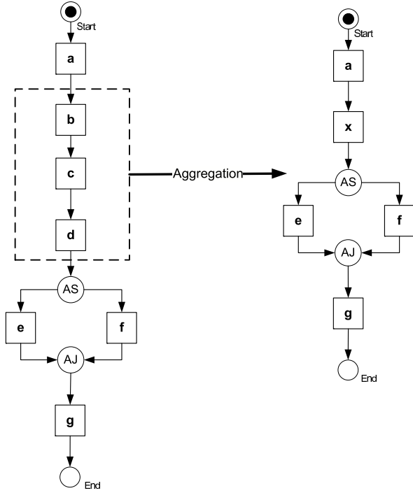
Fig. 6. Application of aggregation
