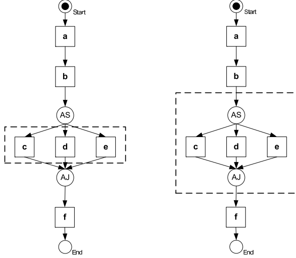
Fig. 4. Left: A wrongly aggregated activity, Right: A correctly aggregated activity
