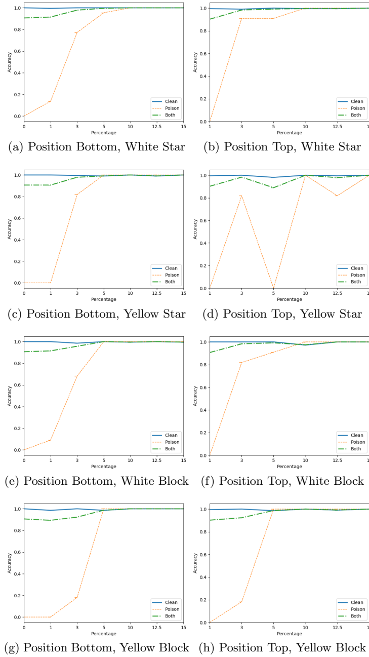
Fig. 4. Results for different positions of the backdoor key on the Belgian dataset: the left column shows the results for the backdoor on the bottom, right on the top
