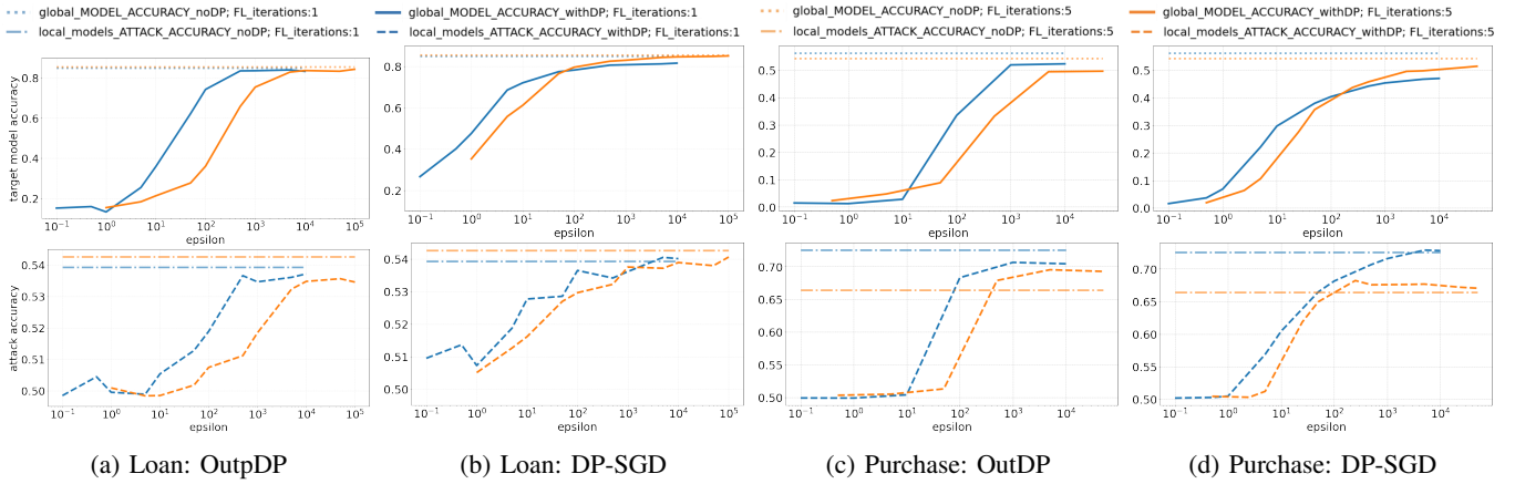
Fig. 1: Output DP and DP-SGD (2 nodes in FL) performance comparison based on global model accuracy and attack accuracy against local models, on different numbers of FL iterations. The colour indicates the point of testing (blue: results after the first federated iteration; orange: results after the fifth federated iteration); dotted lines indicate the baseline when no DP is applied.
