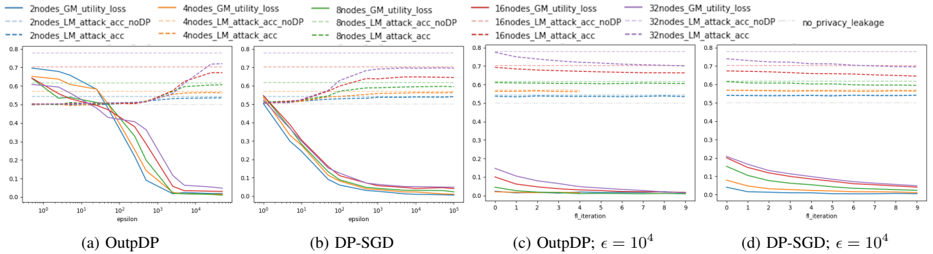
Fig. 2: Output DP and DP-SGD performance on Loan dataset in FL settings with a different number of nodes depending on \epsilon (a,b) and FL iterations (c,d). The global model’s utility loss (GM_utility_loss) is computed as the difference between the global model’s accuracy in FL without DP and with the corresponding DP approach. LM_attack_acc denotes the mean attack accuracy of all local models in the FL setting.
